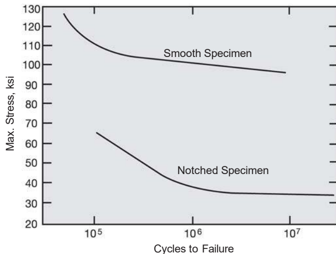
Figure 5. Pull-pull fatigue strength of 1-in. hot-rolled rod equalized and precipitation-treated (1625°F/24 hr, A.C., + 1300°F/20 hr, A.C.).
