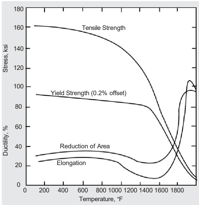
Figure 10. High-temperature tensile properties of bar triple-heat-treated (2100°F/2 hr, A.C., + 1550°F/24 hr, A.C., + 1300°F/20 hr, A.C.).
