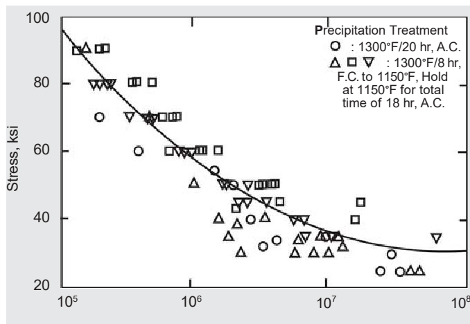
Figure 22. Fatigue strength of cold-rolled annealed sheet (Krouse tests, completely reversed bending).
